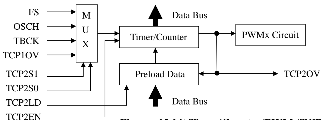
Figure: 12-bit Timer/Counter/PWM (TCP2)
